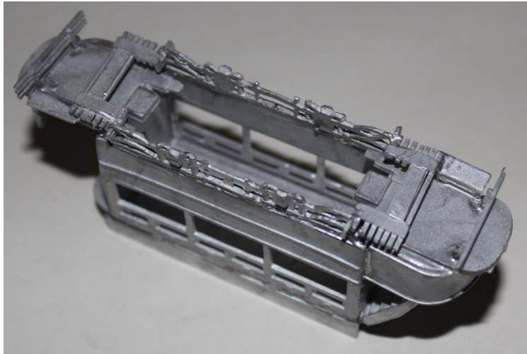
11. Fit the stairs, resistance boxes under the stairs and trolley mast
