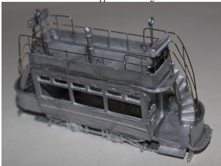
12. Make upper deck rails and hand rails from fine wire. 13. Fix destination boxes to upper deck railings.
