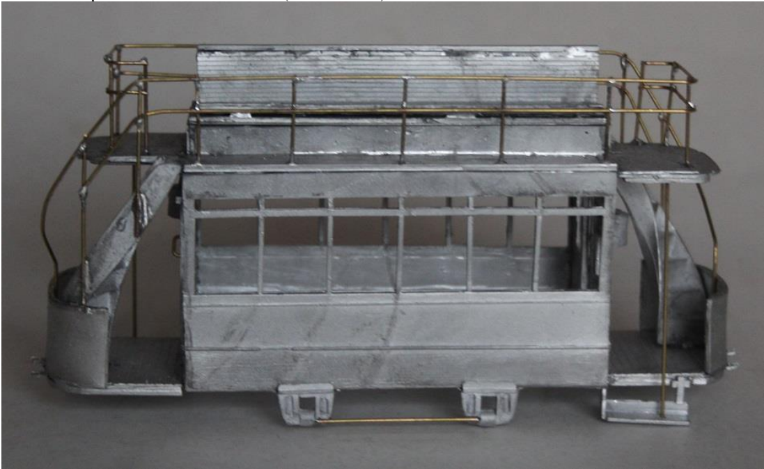
16. Make up handrails etc from wire (not included).
